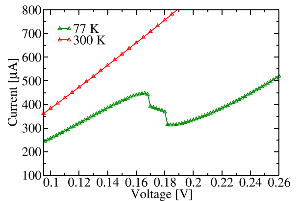
FIG. 2. Experimental I – V characteristics for the \text{Al}_{0.18}\text{Ga}_{0.82}\text{N} RTD with a 49 Å well and mesa size of 4 \times 4 \mu\text{m}^2 at 77 and 300 K. The positive polarity refers to positive bias applied to the top of the mesa and corresponds to electron injection from the left side in Fig. 1.
